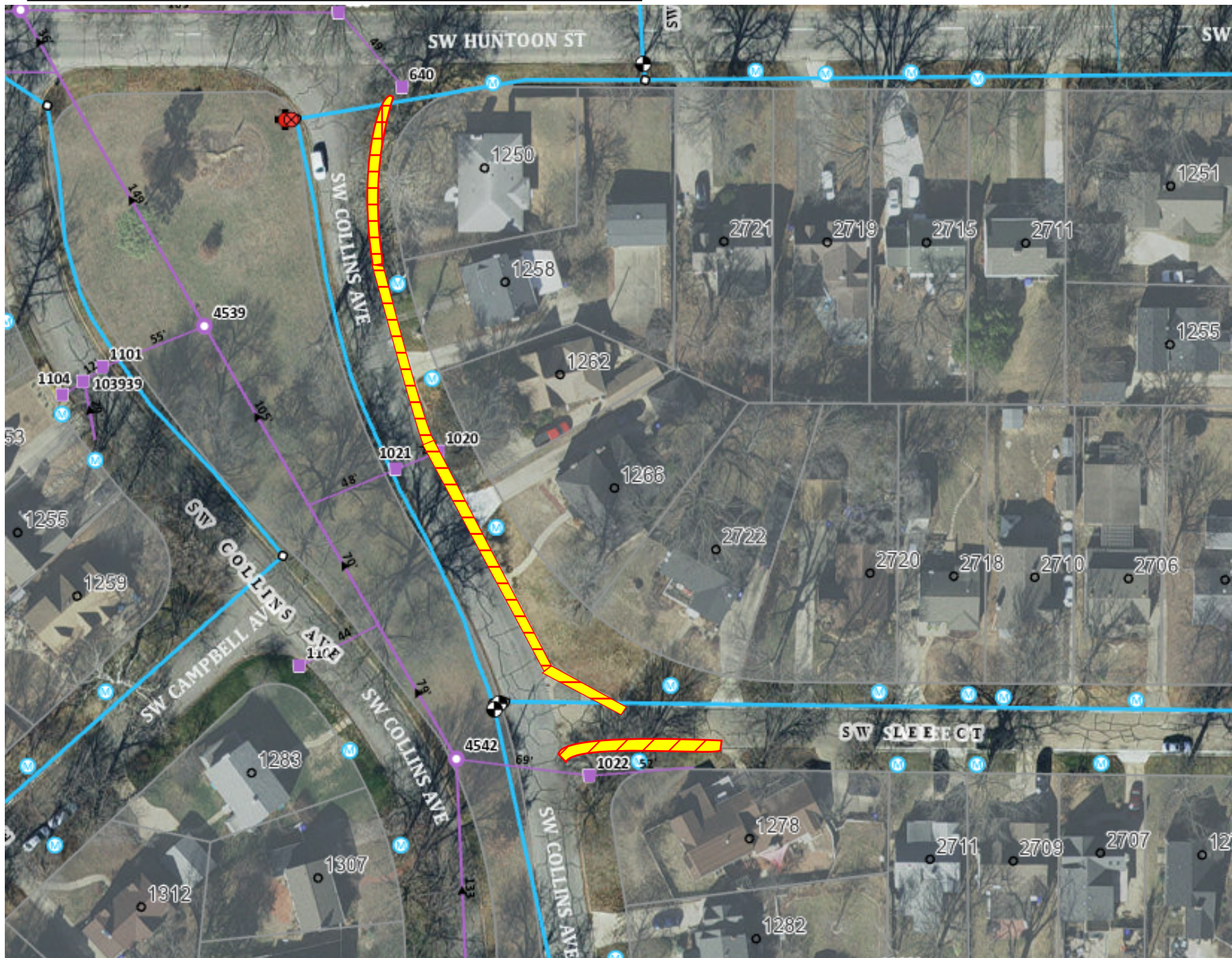
841102.01 Collins Park Phase II Curb & Gutter Location Map
