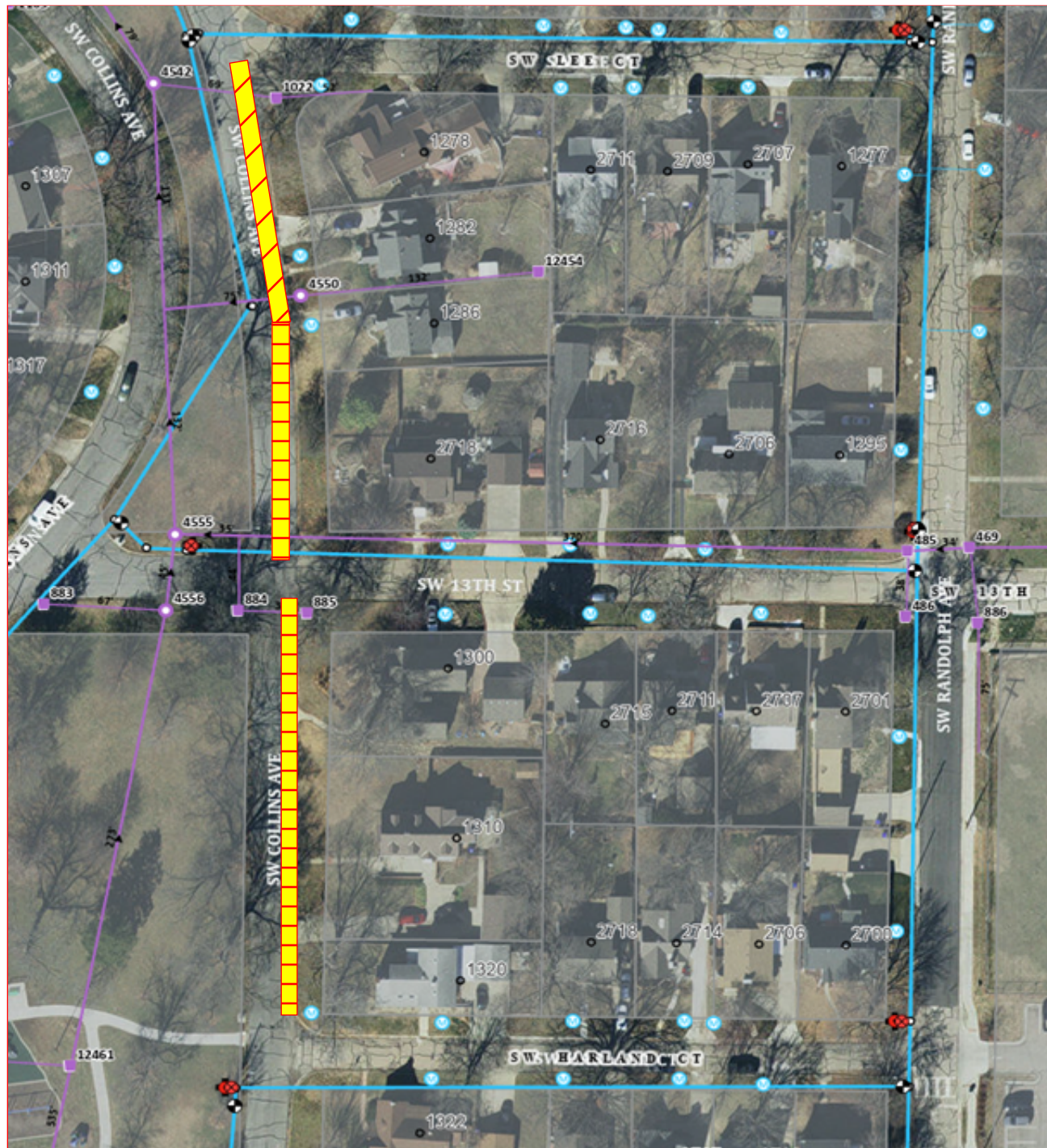
841102.01 Collins Park Phase II Curb & Gutter Location Map
